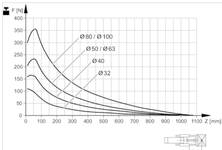
Service life 5 \times 10^6 m F = Useful load, Z = Projection
