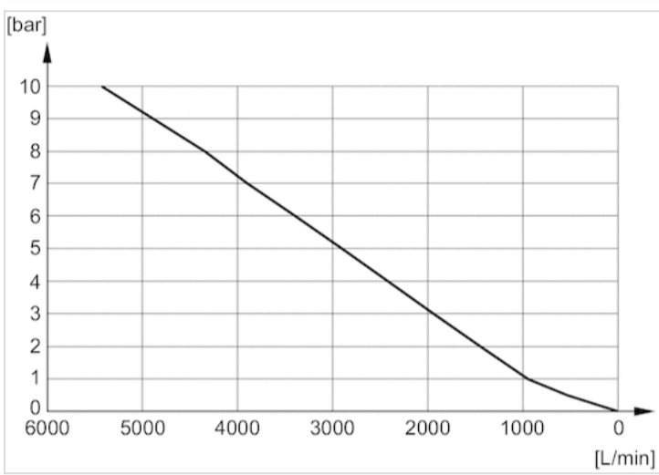
Flow diagram 1827000002
