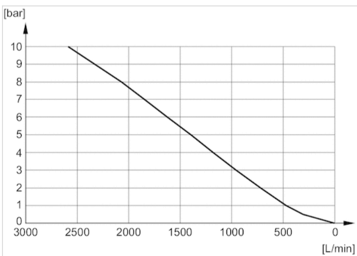
Flow diagram 1827000000
