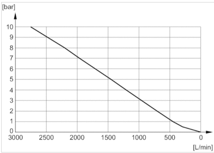
Flow diagram 1827000035
