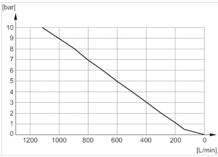
Flow diagram 1827000033
