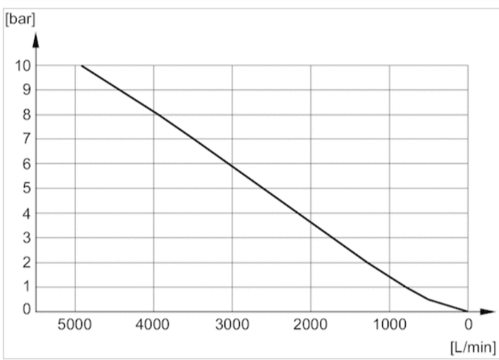
Flow diagram 5324001120
