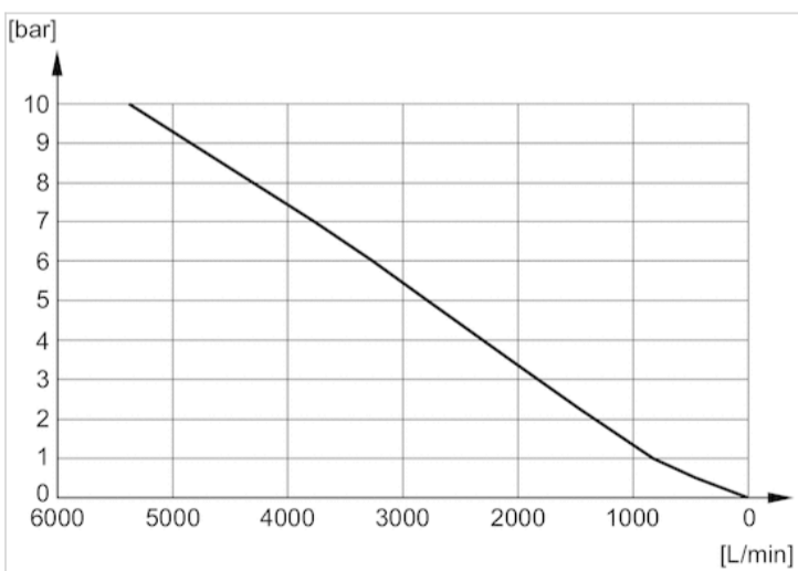
Flow diagram 8145003400
