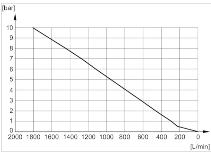
Flow diagram 1827000034
