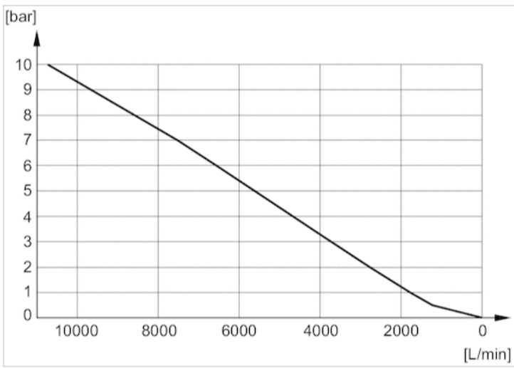
Flow diagram 1827000003
