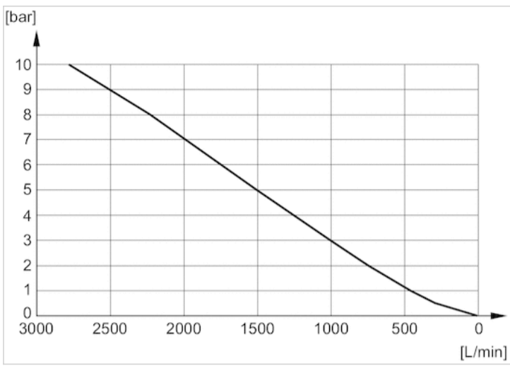
Flow diagram 5324001170
