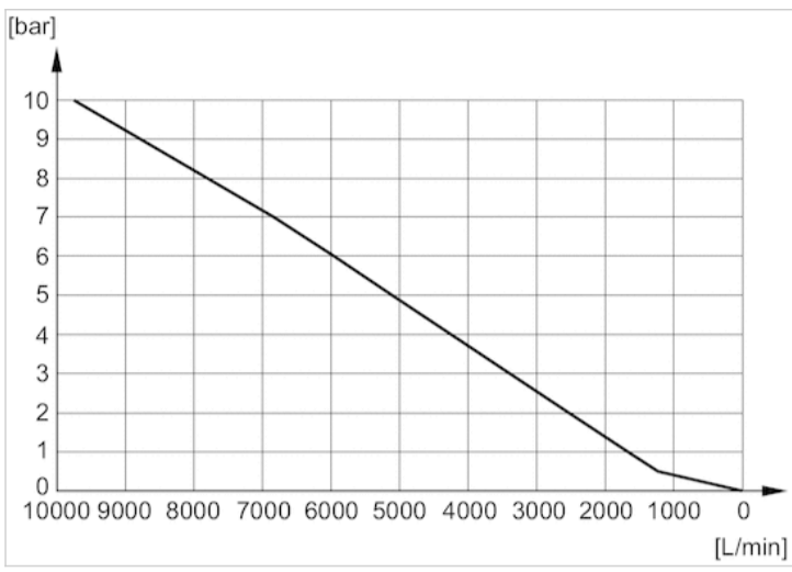
Flow diagram 1827000001
