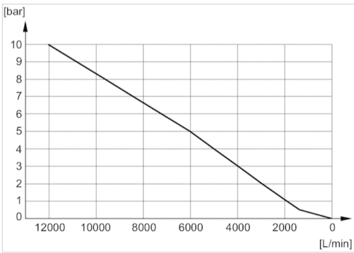
Flow diagram 1827000004
