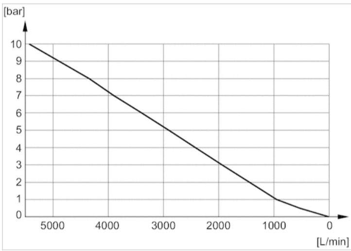
Flow diagram 5324001140
