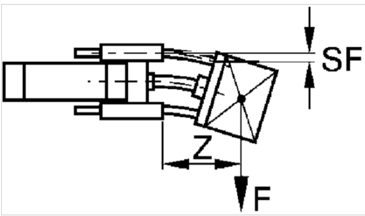
F = useful load (at the load center), SF = bending, Z = projection
